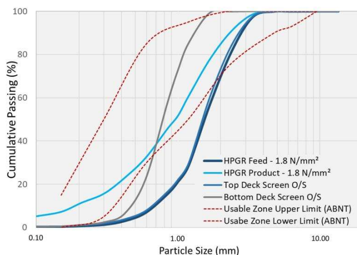
Figure 10. Survey 4 size distributions and limits for use as sand for concrete.
