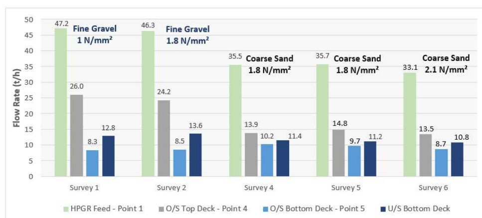
Figure 6. Summary of mass balance results.
