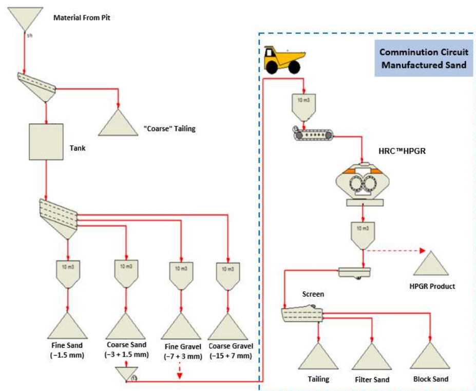
Figure 2. Itaquareia processing plant flow sheet.
