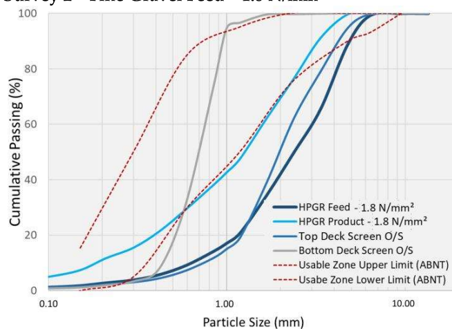
Figure 9. Survey 2 size distributions and limits for use as sand for concrete.
