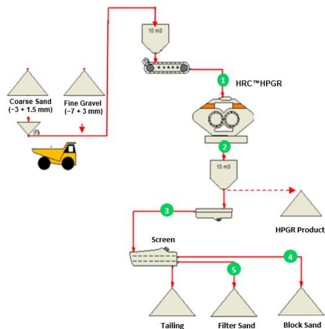
Figure 5. Itaquareia comminution circuit and sampled streams.
