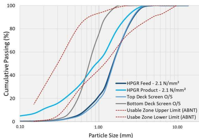
Figure 11. Survey 6 size distributions and limits for use as sand for concrete.
