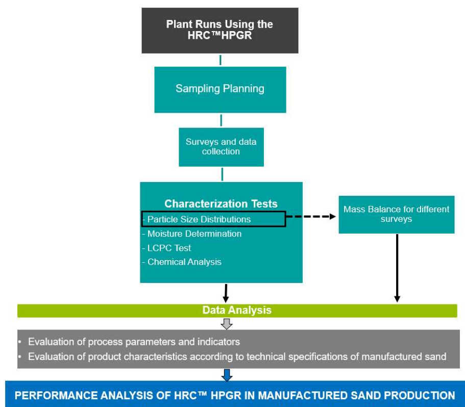
Figure 4. Method adopted for assessing the performance of HRC™ in the Itaquareia industrial processing plant.
