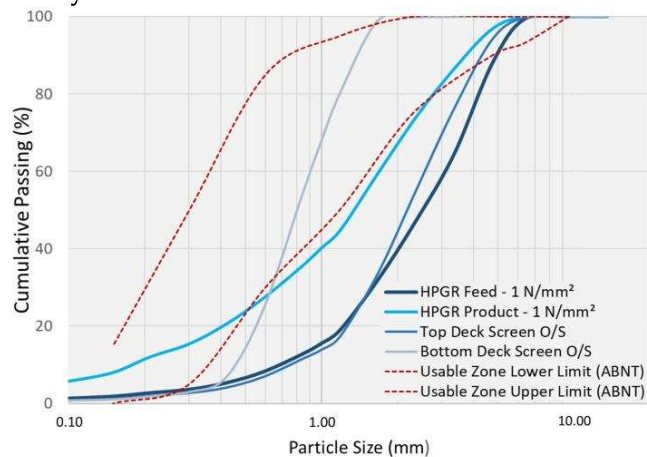
Figure 8. Survey 1 size distributions and limits for use as sand for concrete.
